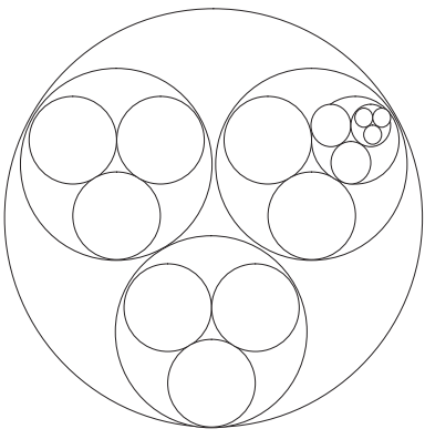
Fig. 1. Schematic cross section of multiple triple strand.
